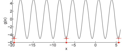
Figure 3. Typical failing of unscented filters. Although the function highly varies, the sigma points (red dots) are mapped to almost the same function value (red crosses). The sample predictive distribution is overconfident.
